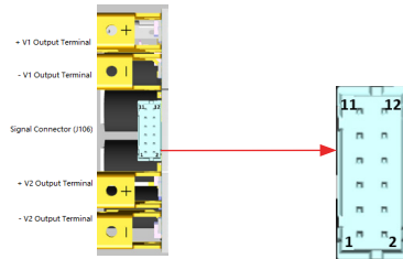
J106 Signal Connector - Dual Output Module
